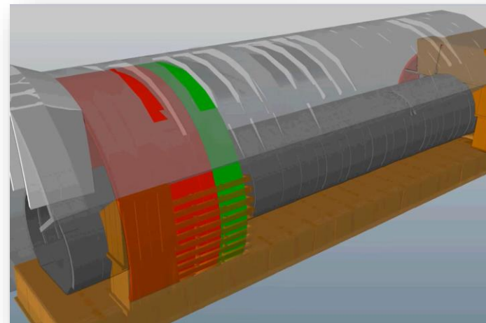
Headwall construction
