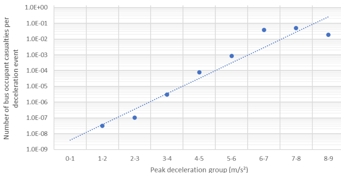
Figure 51: Relationship between casualties per event and peak deceleration
