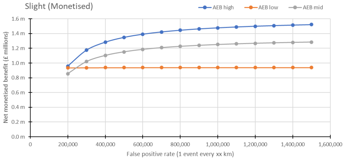
Figure 34: The effect of false positive rate on the annual net monetised benefit of each candidate AEB system (central prediction) for slight casualties only (Using updated data from CCTV and telematics analysis and adjusted for empty buses)
