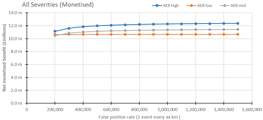
Figure 31: The effect of false positive rate on the annual net monetised benefit of each candidate AEB system (central prediction) (Using updated data from CCTV and telematics analysis and adjusted for empty buses)
