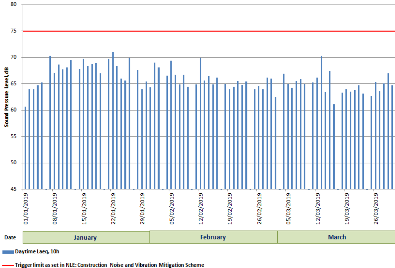
Noise Time History: Receptor R1 - Sherwin House
