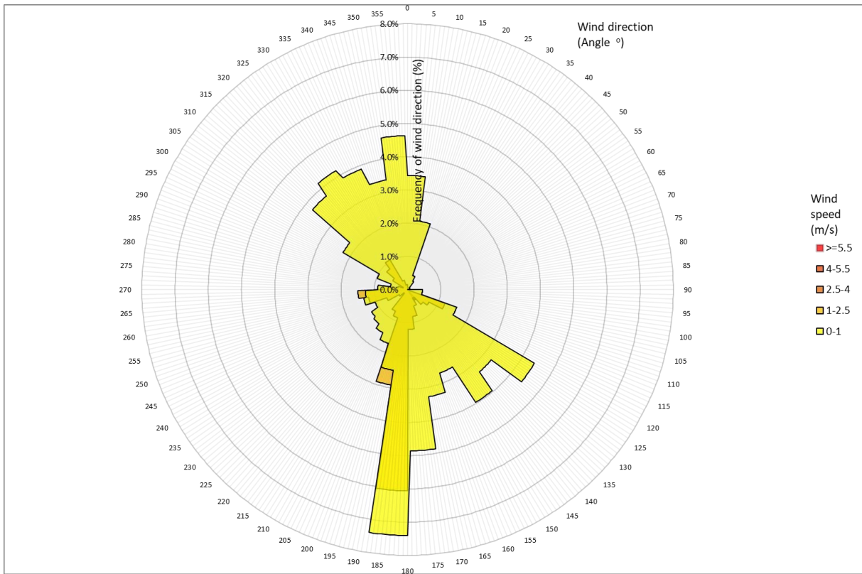
Figure 1. Wind rose from the Battersea sonic anemometer BN2W. Period 1.
