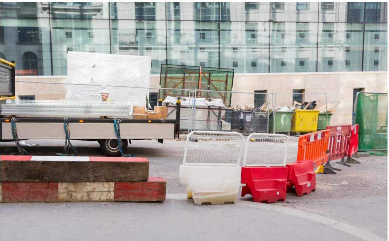
Bad practice: multitude of mixed barrier types, which are not assembled into a continuous barrier
