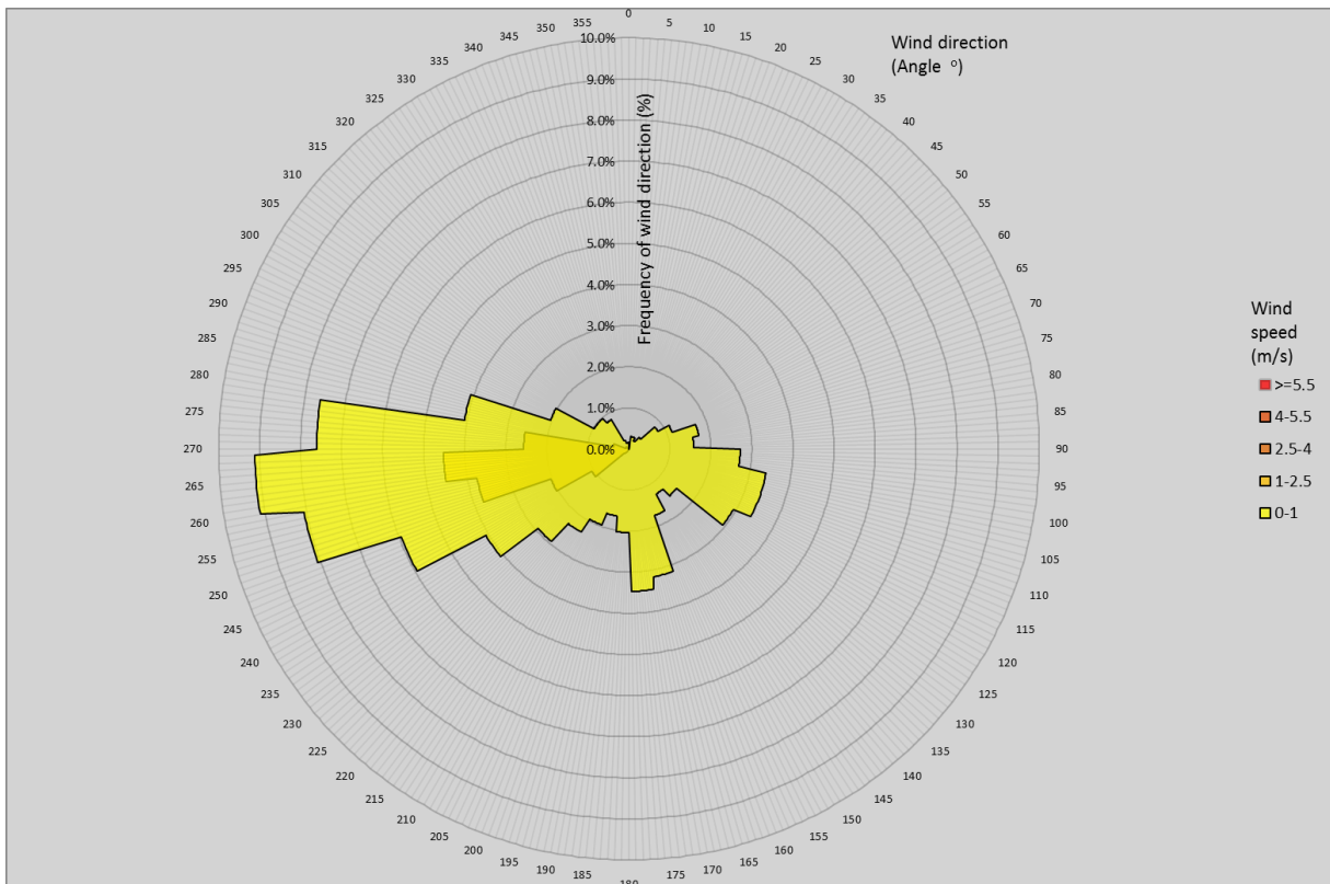
Figure 2. Wind rose from the Kennington Park sonic anemometer KP2W. Period 2.
